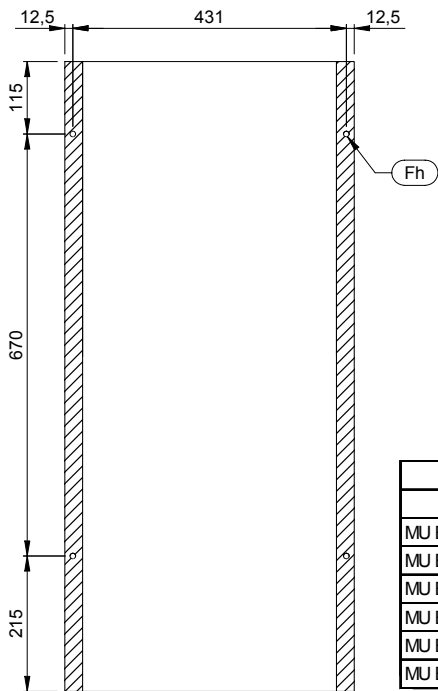
IMPRONTA A PARETE / WALLPRINT
