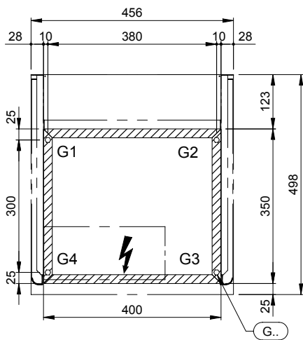
IMPRONTA A TERRA / FOOTPRINT
